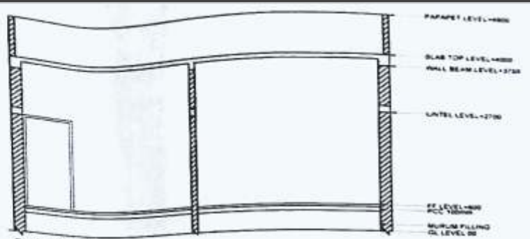
SECTION XY
